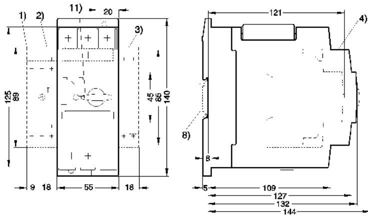
Moulded plastic front plate J74MN-P12
